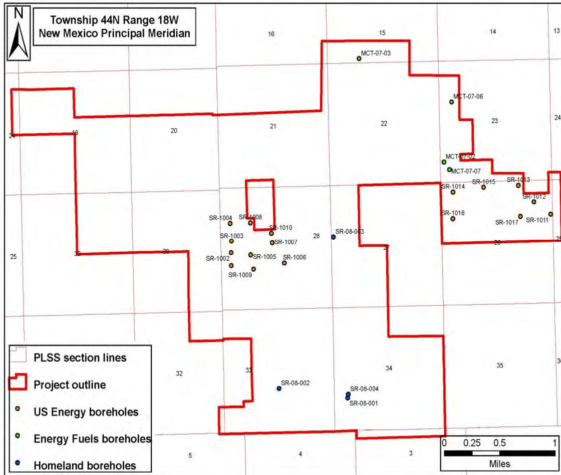
Figure 6.1 - 2006-2008 Borehole Map
