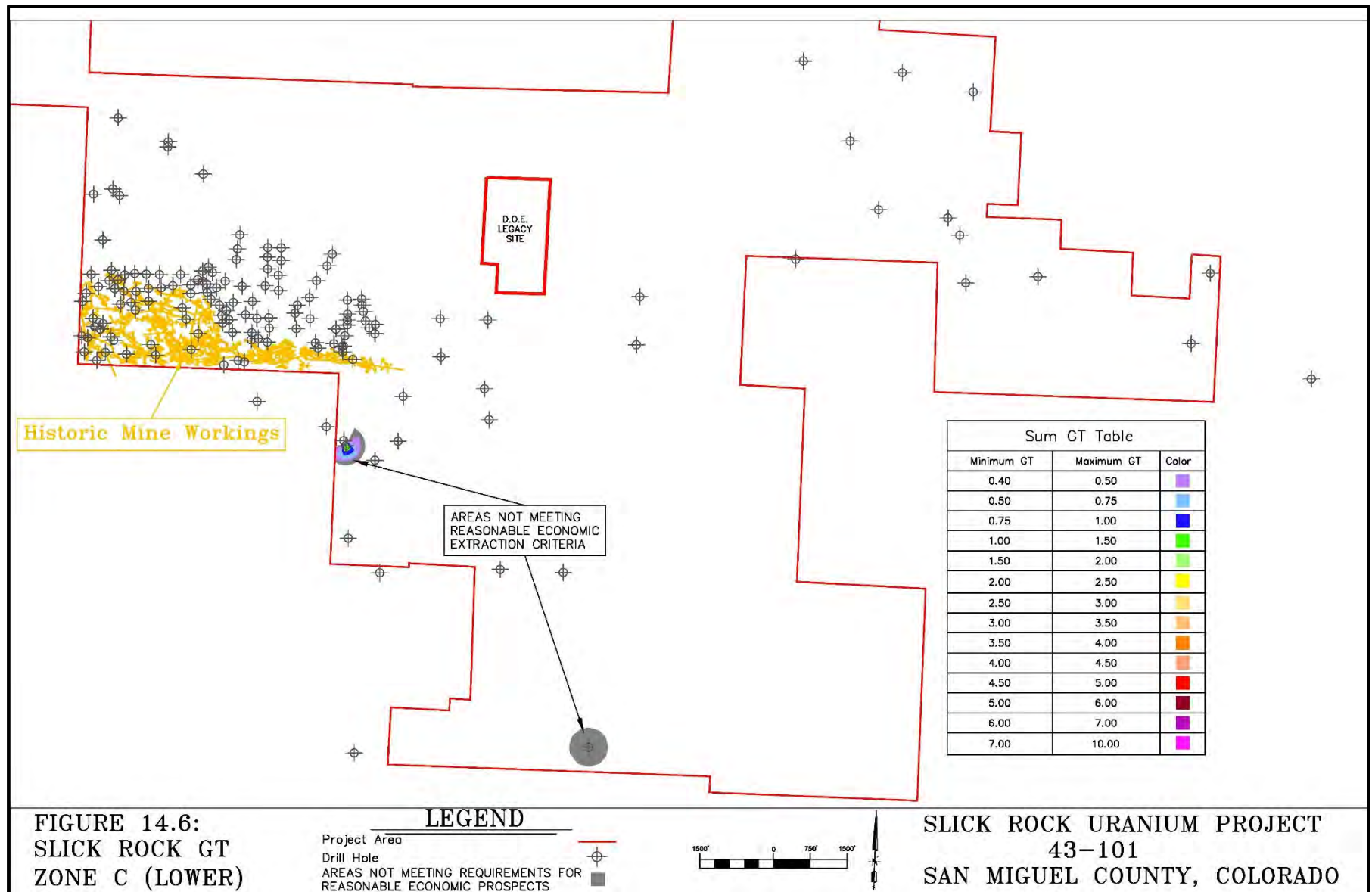
Figure 14.6 - Slick Rock Zone C GT Map
